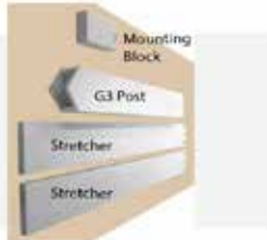
Prestige Gable Detail dimensions: 4" x 12" actual size, 4" x 10" actual is also available.
