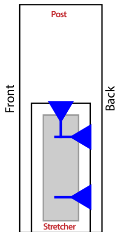
Assembly Fastener layout Side view
