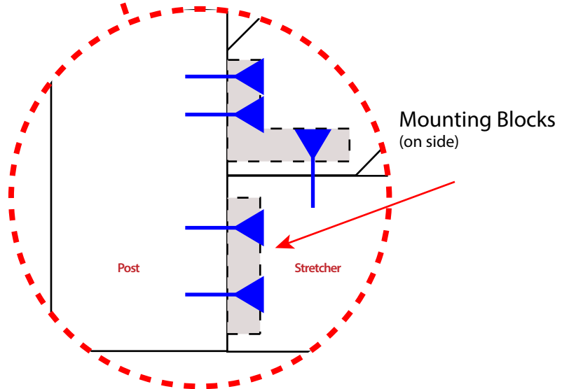
Assembly Fastener layout Side view
