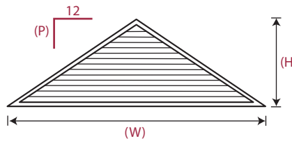
D-37 TRIANGLE LCP3F-PW(H) *S,3,5,7,1
