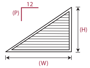
D-40 1/2 TRIANGLE LCP3N-PW(H) *S,3,5,7,1
